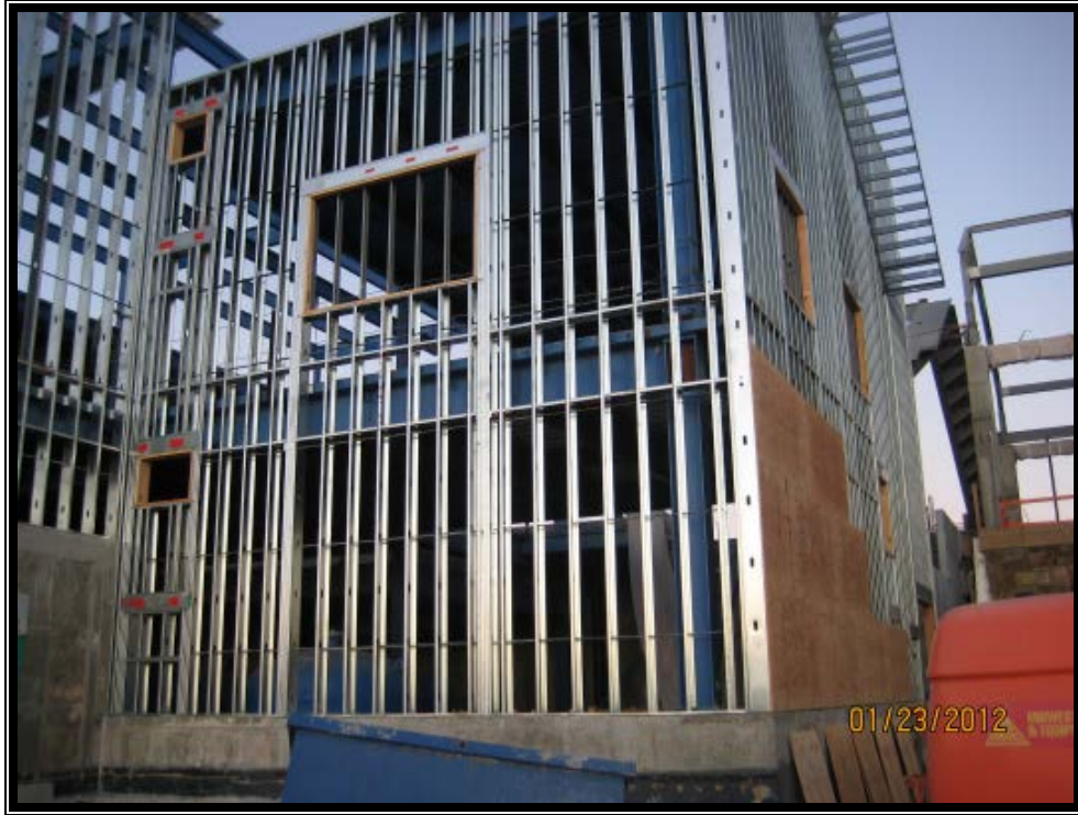
BOH Exterior Studs/Sheathing
